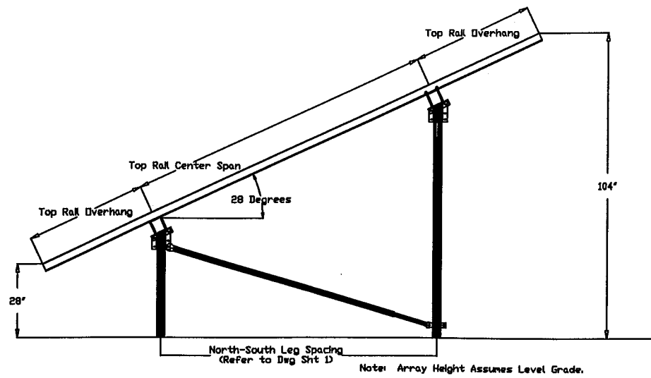
SIDE ELEVATION DETAIL
