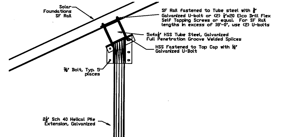
UPPER CAP DETAIL
