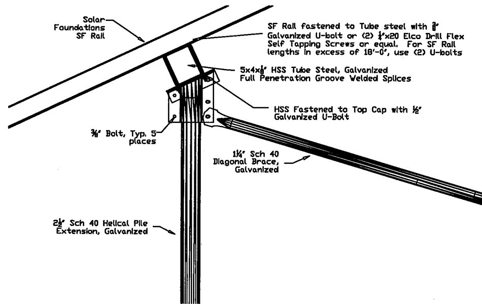
SIDE ELEVATION DETAIL
